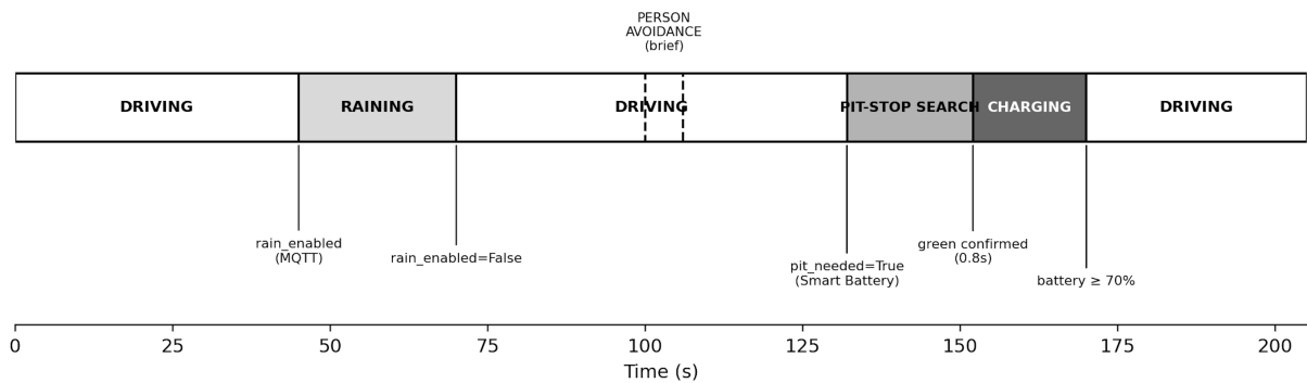
Figure 3 Observed mode timeline for a representative run, showing rain-mode activation, a brief person-safety interruption, and a Smart-Battery-triggered pit stop and recharge.
